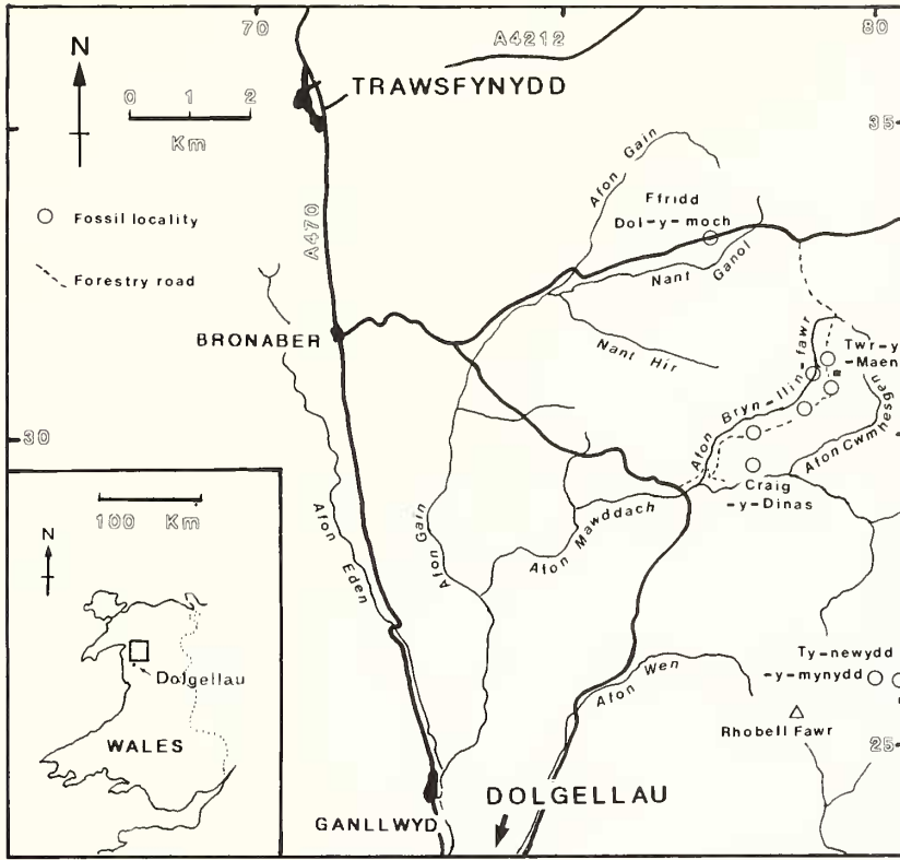
TEXT-FIG. 1. Localities of Cambrian tergomyan molluscs described in the text (modified from Allen et al. 1981).
